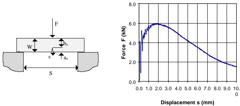
Figure 1 - Mechanical system (left) and the corresponding force-displacement diagram (right) of a bending test with an edge-cracked specimen in the upper-shelf range.
