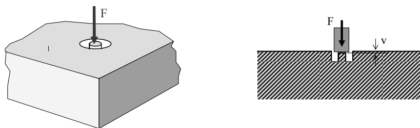
Fig. 5: Mechanical system of the pin compression test
