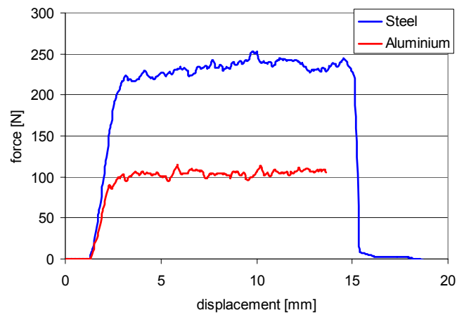
Fig. 8: Examples of measured force-vs.-displacement curves
