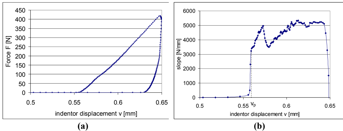
Fig. 3: Example of an indentation curve obtained by a ball indentation test on stainless steel 316L using a sapphire ball with D=1.0\text{mm} (a) and the corresponding slope with definition of v_p (b)
