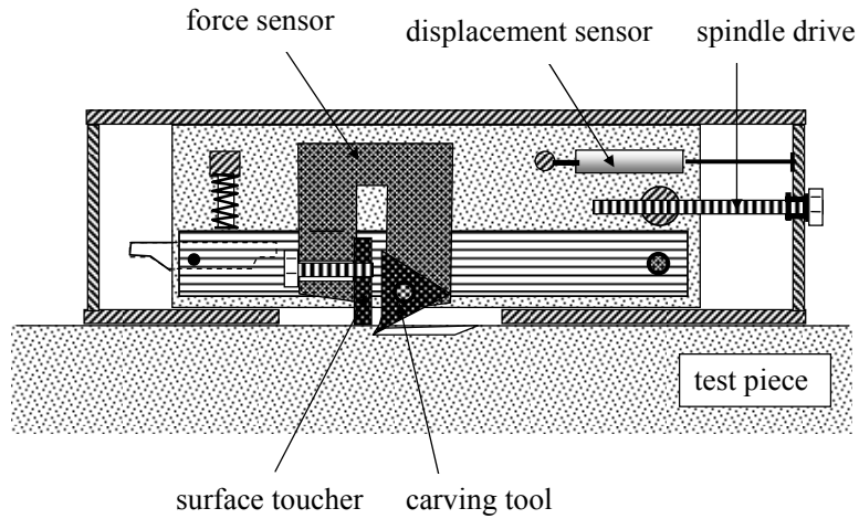
Fig. 7: Principle of the Mat-Tec Carver
