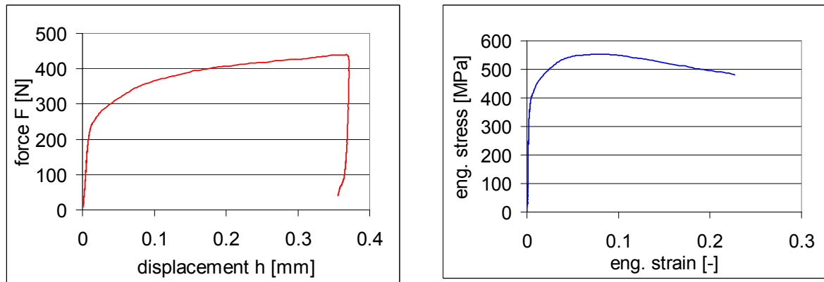
Fig. 6: Example (Steel Fe 510, pin-diameter 0.88 mm, pin length 2.3 mm) of a force-displacement-diagram of a pin compression test and the corresponding stress-strain diagram
